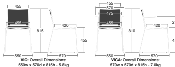
VIC: Overall Dimensions: 550w x 570d x 815h - 5.8kg
